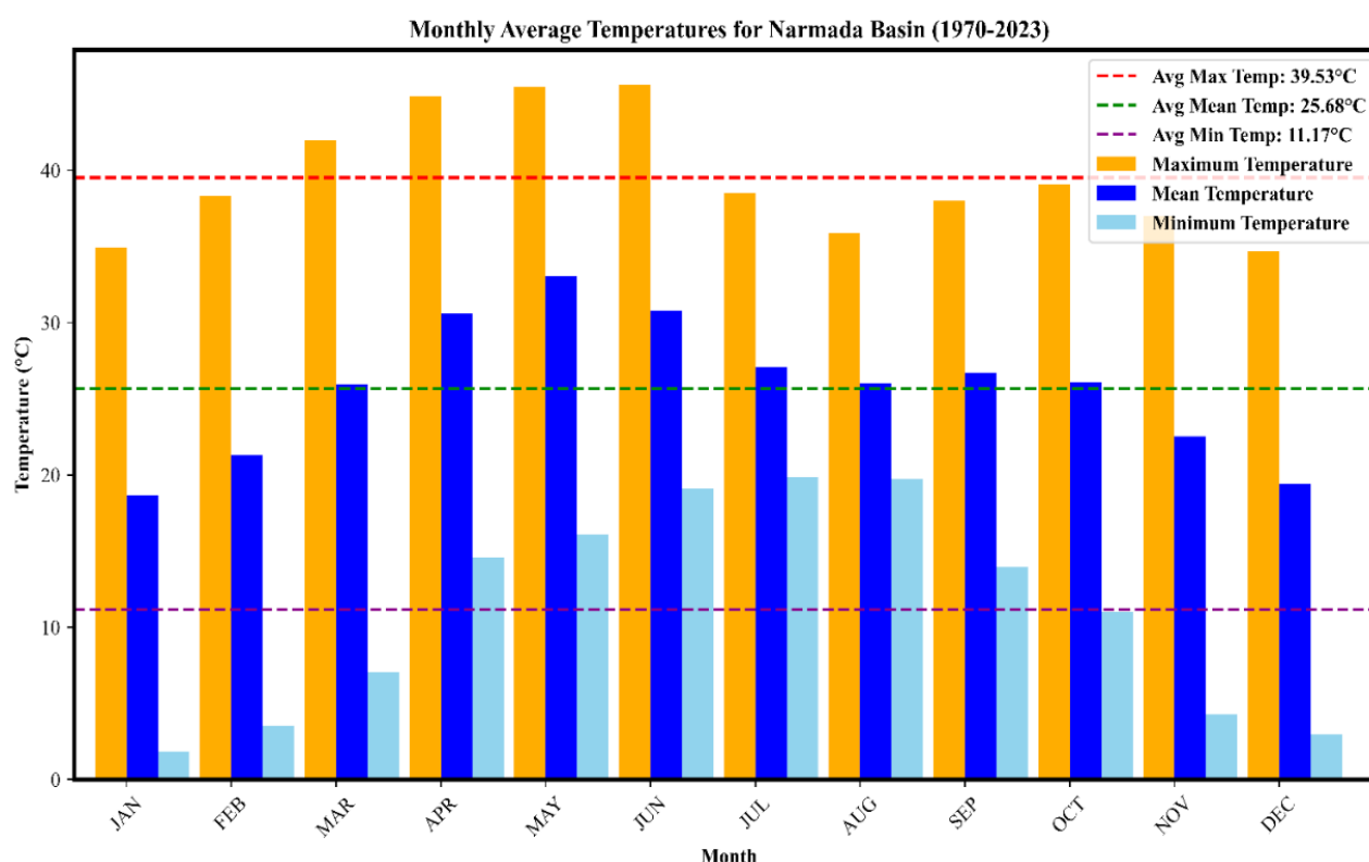
Figure 9 Trends in monthly average temperature (1970 -2023)
