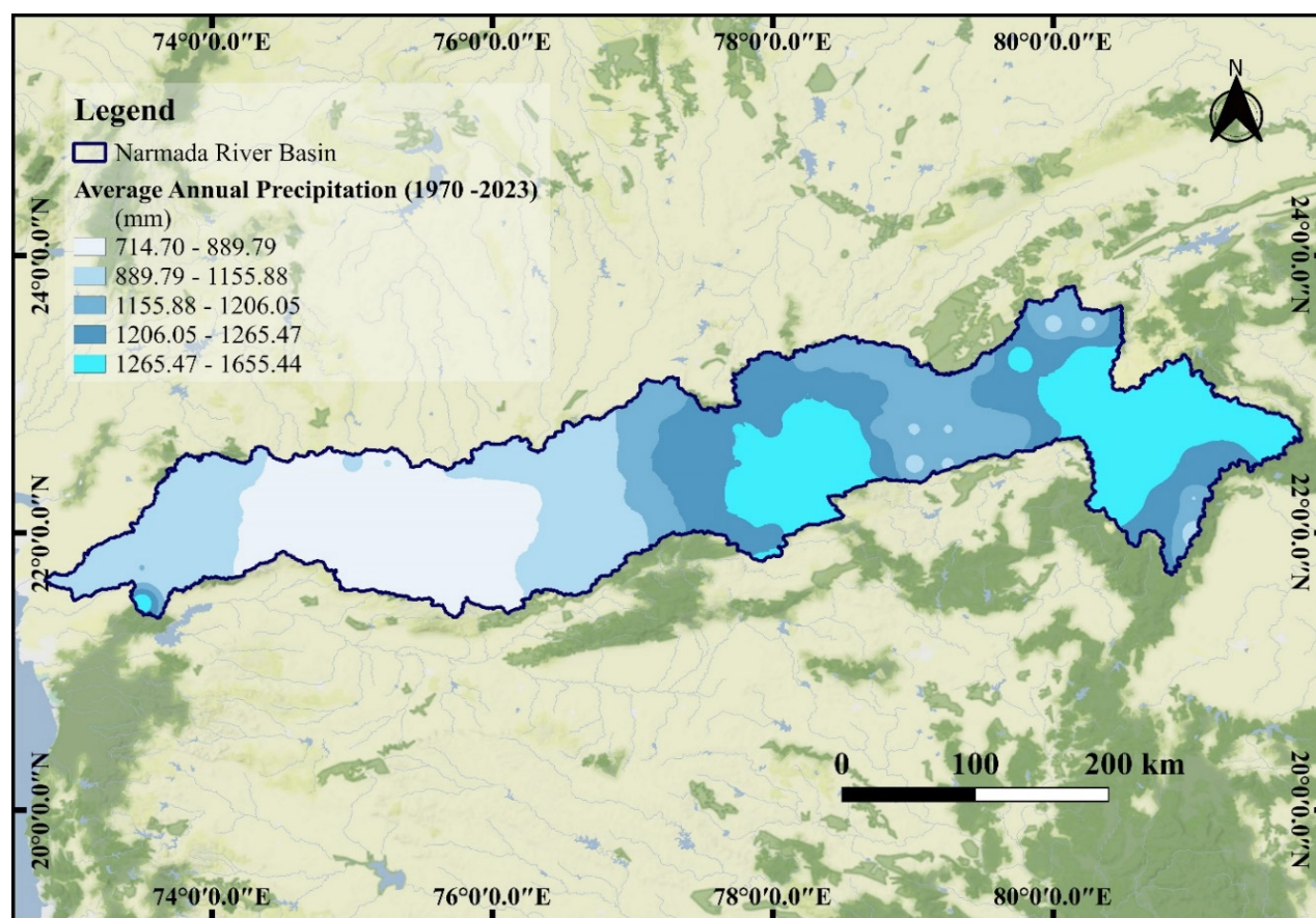
Figure 6 Spatial distribution of precipitation (1970 – 2023) Source: IMD gridded data (0.25° X 0.25°)
