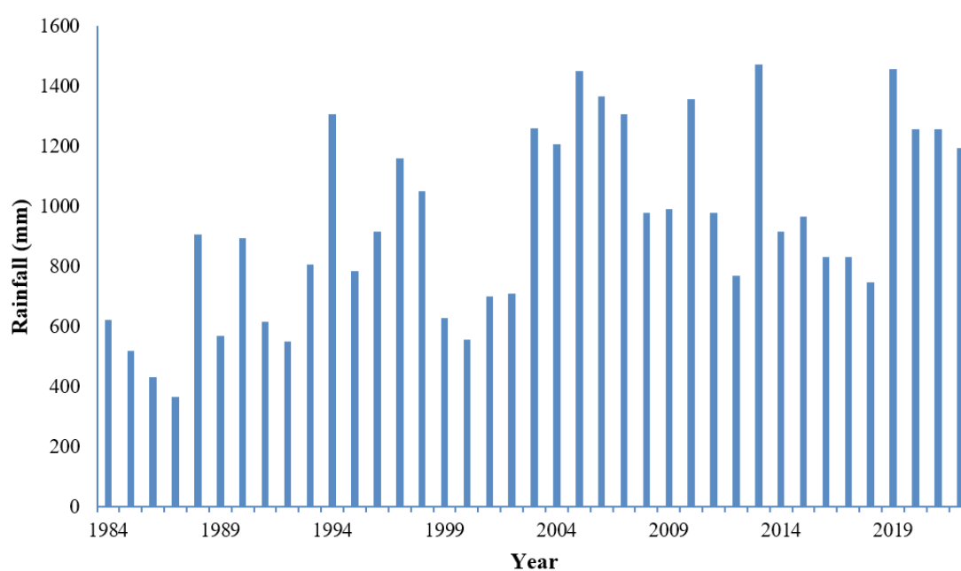
Figure 44 Variation of average annual rainfall over the Lower Narmada Basin
