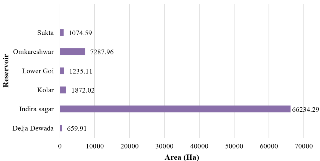
Figure 30 Reservoirs in the Middle Narmada Basin segment
