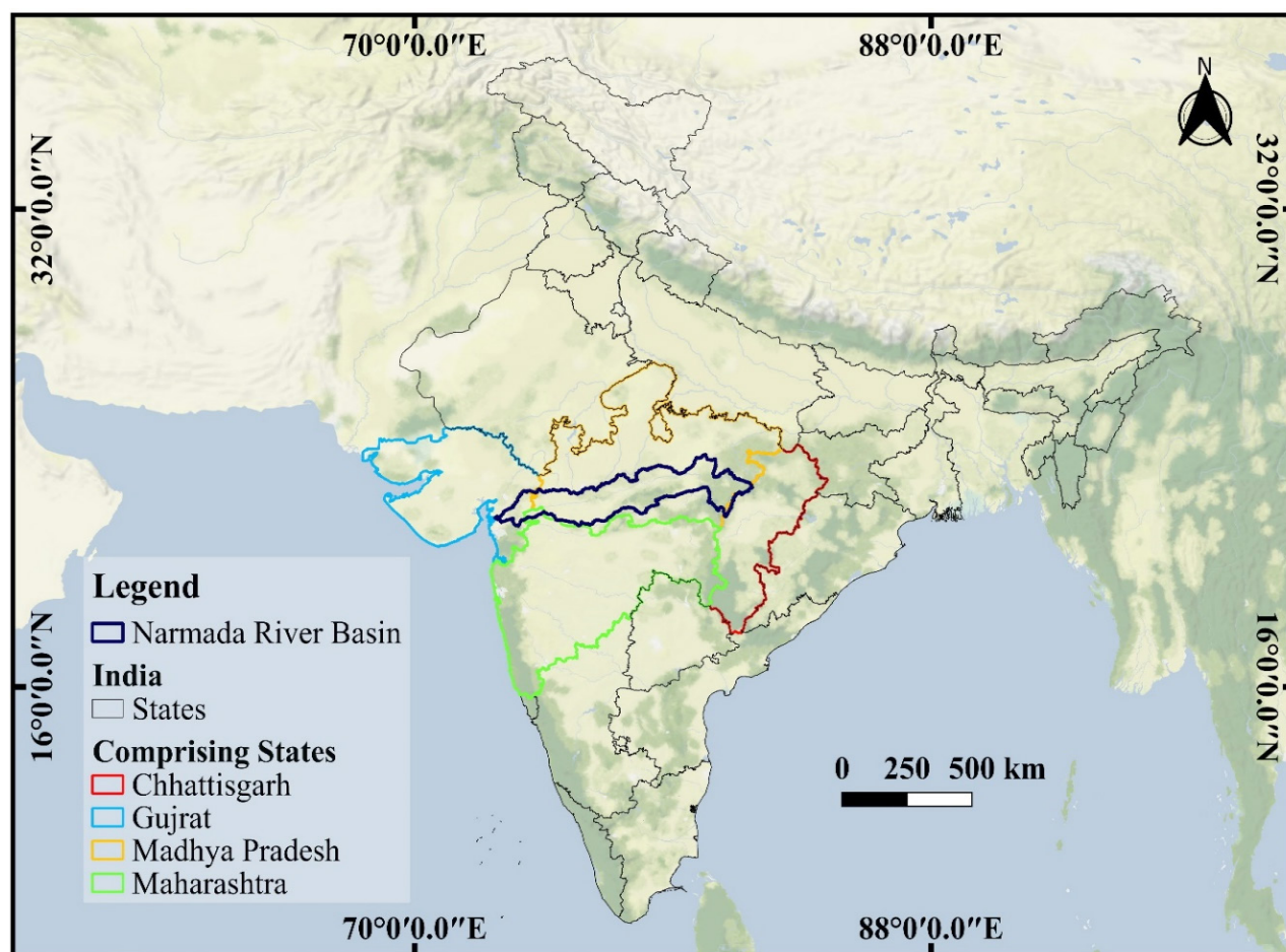
Figure 1 Geographical location map
