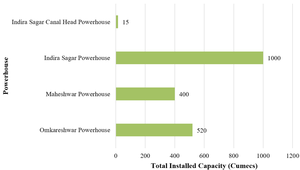
Figure 31 Powerhouses in the Upper Narmada Basin segment
